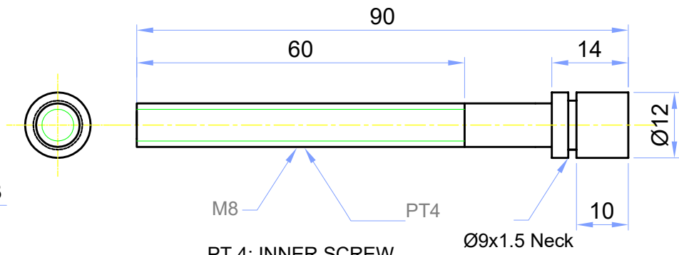
PT 4: INNER SCREW
