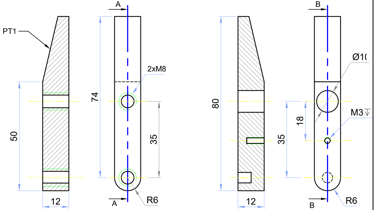
SECTION A-A PT 1: MOVABLE JAW
